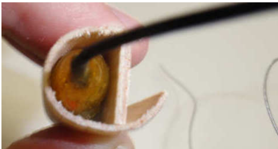
Figure 5 Hold the tube segment against the base with the tx in place. When everything looks and feels right, remove the tx and and CA the two together. The excess tube material can then be trimmed.
